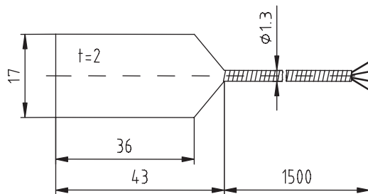
T65.43x17.Sil
