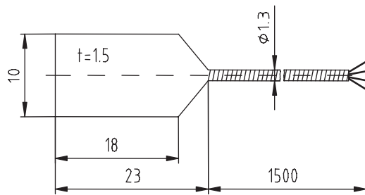
T65.23x10.Sil
