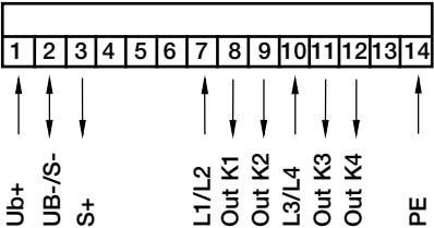
Steckverbinder plugin connector assemblage connector Art.-Nº.: 408837
