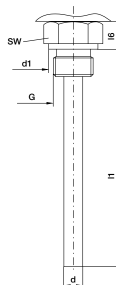
Form 6 Einschraubzapfen fest male thread raccord fixe
