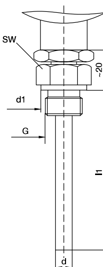
Form 6 Einschraubzapfen fest male thread raccord fixe
