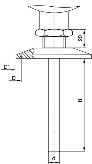
Form FC Tri-Clamp clamp connection raccord clamp
